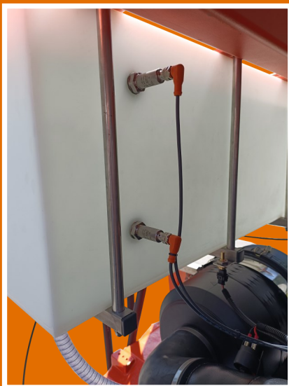
Water level switches
